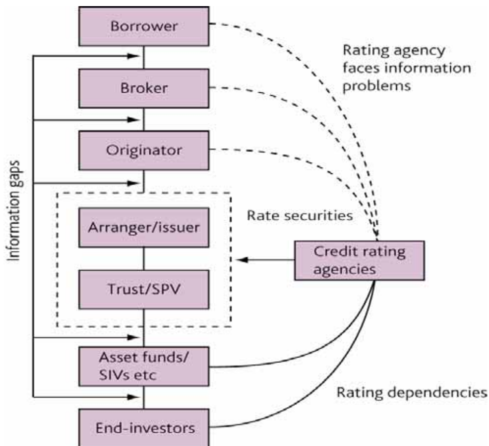
Chart 2 – Information Loss
