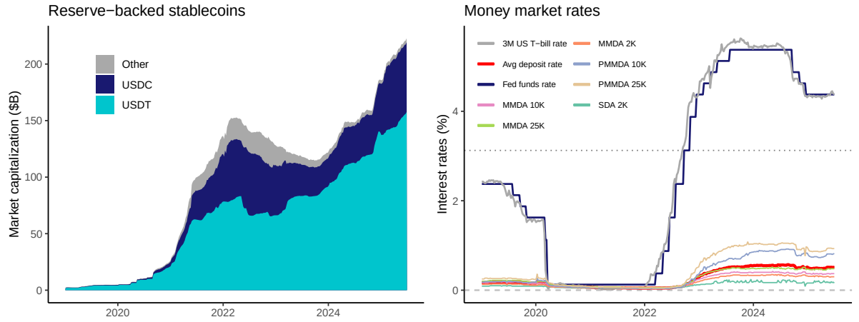
Figure 1: Left: reserve-backed stablecoin market capitalization by issuer (USDT, USDC, and other). Right: federal funds rate, 3-month T-bill rate, average non-maturity deposit rate (red line), and individual deposit rates by tier. Sample: January 2019 – June 2025. The dotted horizontal line indicates a federal funds target rate midpoint of 3.125%.
