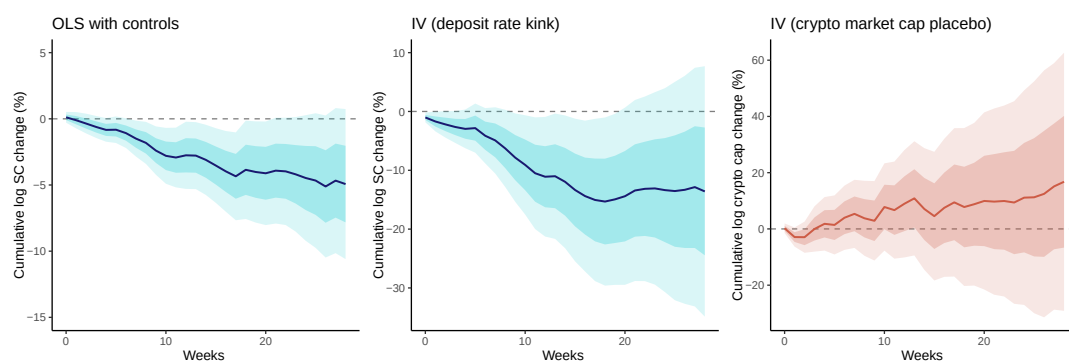
Figure OA.H.1: Full-sample results. Cumulative response to a 1 basis point deposit rate increase. Left: OLS with controls. Center: IV using the deposit rate kink. Right: crypto market placebo for the IV specification. Darker and lighter shaded regions correspond to 68% and 95% Newey-West confidence bands (bandwidth h ).
