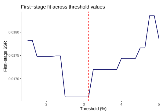
Figure OA.J.2: First-stage sum of squared residuals across candidate thresholds.
