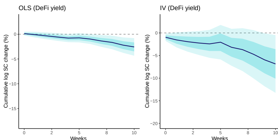
Figure OA.E.1: Full-sample OLS (left) and IV (right) controlling for changes in stablecoin DeFi yields. The yield index is constructed as the equal-weighted average of DeFi yields offered on Dai/USDS and USDC on Aave and Compound, respectively. Darker and lighter shaded regions correspond to 68% and 95% Newey-West confidence bands (bandwidth h ).
