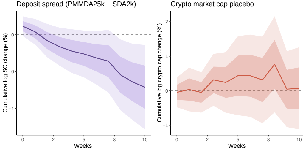
Figure 4: Cross-sectional results. Left: response to deposit rate spread (PMMDA25k – SDA2k). Right: crypto market cap placebo. Darker and lighter shaded regions correspond to 68% and 95% Newey-West confidence bands (bandwidth h ).
