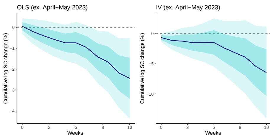
Figure OA.D.1: Full-sample OLS (left) and IV (right) excluding April–May 2023. Darker and lighter shaded regions correspond to 68% and 95% Newey-West confidence bands (bandwidth h ).
