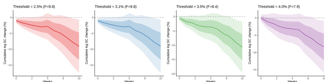
Figure OA.J.1: Full-sample IV at alternative thresholds. First-stage F -statistics reported in panel titles. Darker and lighter shaded regions correspond to 68% and 95% Newey-West confidence bands (bandwidth h ).
