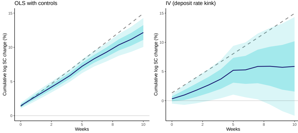
Figure 6: OLS (left) and IV (right) estimates plotted against average cumulative stablecoin growth (dashed line). The solid line and shaded bands show the implied growth path after a 1 basis point deposit rate increase. Darker and lighter shaded regions correspond to 68% and 95% Newey-West confidence bands (bandwidth h ).
