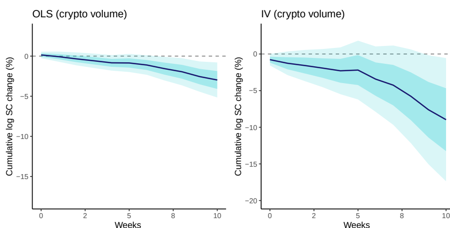
Figure OA.B.1: Full-sample OLS (left) and IV (right) controlling for log of the 7-day average aggregate cryptocurrency trading volume sourced from CoinGecko. Darker and lighter shaded regions correspond to 68% and 95% Newey-West confidence bands (bandwidth h ).
