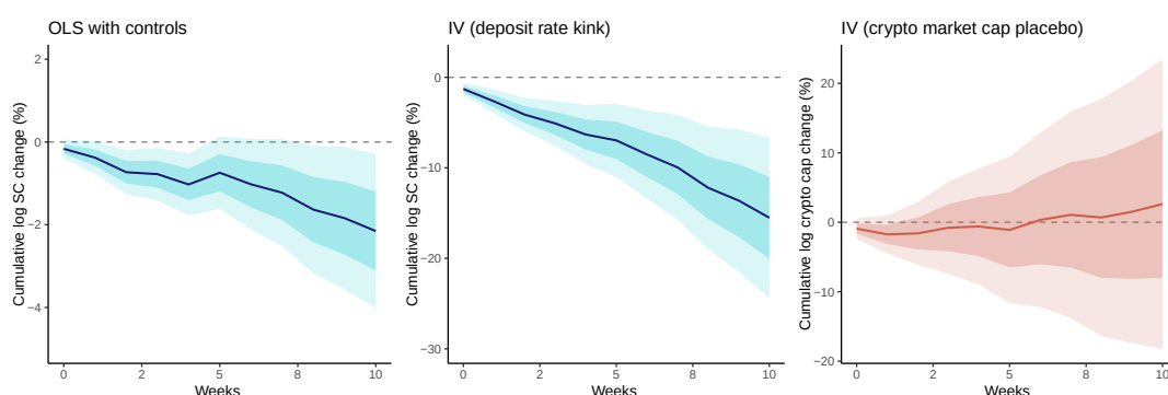
Figure OA.G.1: Full-sample results. Cumulative response to a 1 basis point CD rate increase. Left: OLS with controls. Center: IV using the deposit rate kink. Right: crypto market placebo for the IV specification. Darker and lighter shaded regions correspond to 68% and 95% Newey-West confidence bands (bandwidth h ).
