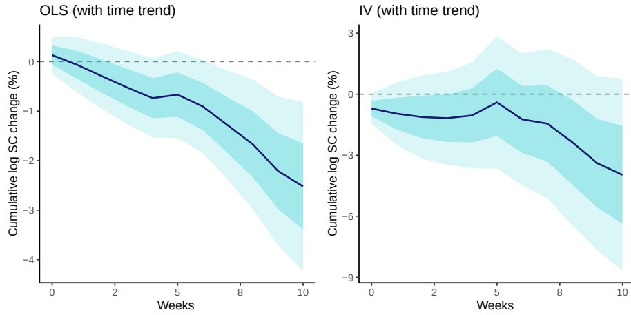
Figure OA.I.1: Full-sample OLS (left) and IV (right) with a linear time trend. Darker and lighter shaded regions correspond to 68% and 95% Newey-West confidence bands (bandwidth h ).
