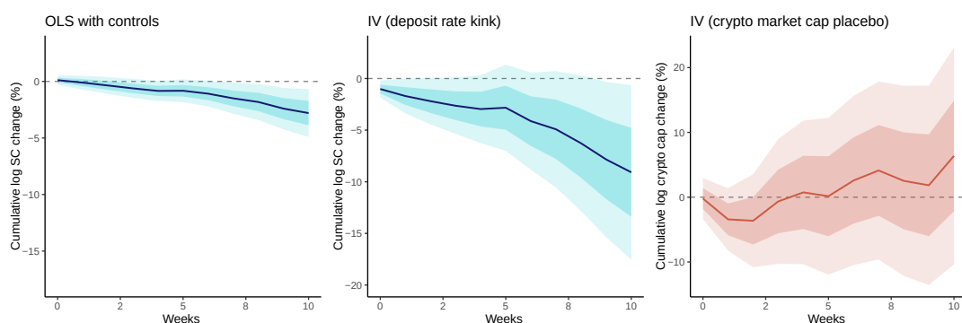
Figure 3: Full-sample results. Cumulative response to a 1 basis point deposit rate increase. Left: OLS with controls. Center: IV using the deposit rate kink. Right: crypto market placebo for the IV specification. Darker and lighter shaded regions correspond to 68% and 95% Newey-West confidence bands (bandwidth h ).
