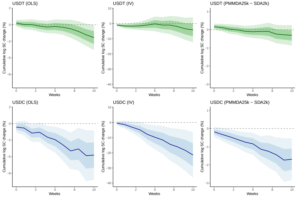
Figure 5: OLS, IV and deposit spread estimates by stablecoin. Top: Tether’s USDT. Bottom: Circle’s USDC. Darker and lighter shaded regions correspond to 68% and 95% Newey-West confidence bands (bandwidth h ).
