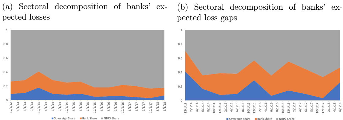
Figure 1: Sectoral decompositions
