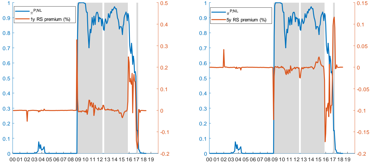
Figure 8: Regime-shift risk premium (monthly return) and \mathbb{P} transition probability
