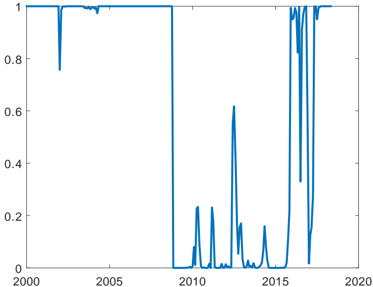
Figure 7: Filtered N -regime probability
