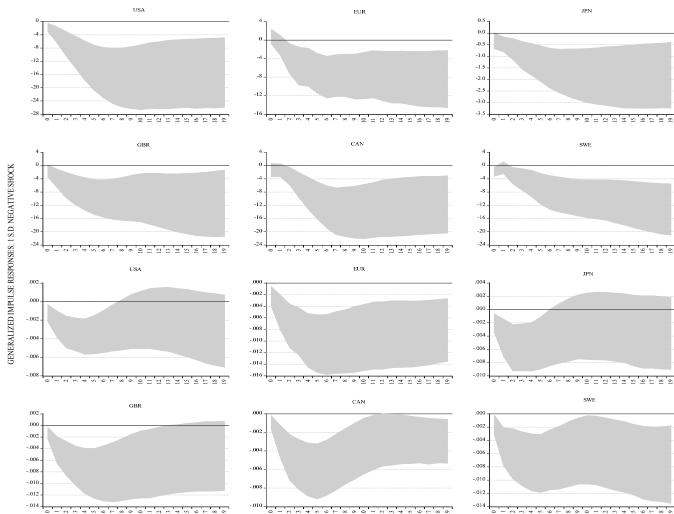
Figure 8A Impulse Responses to a Negative Loan Demand Shock from the Euro area
