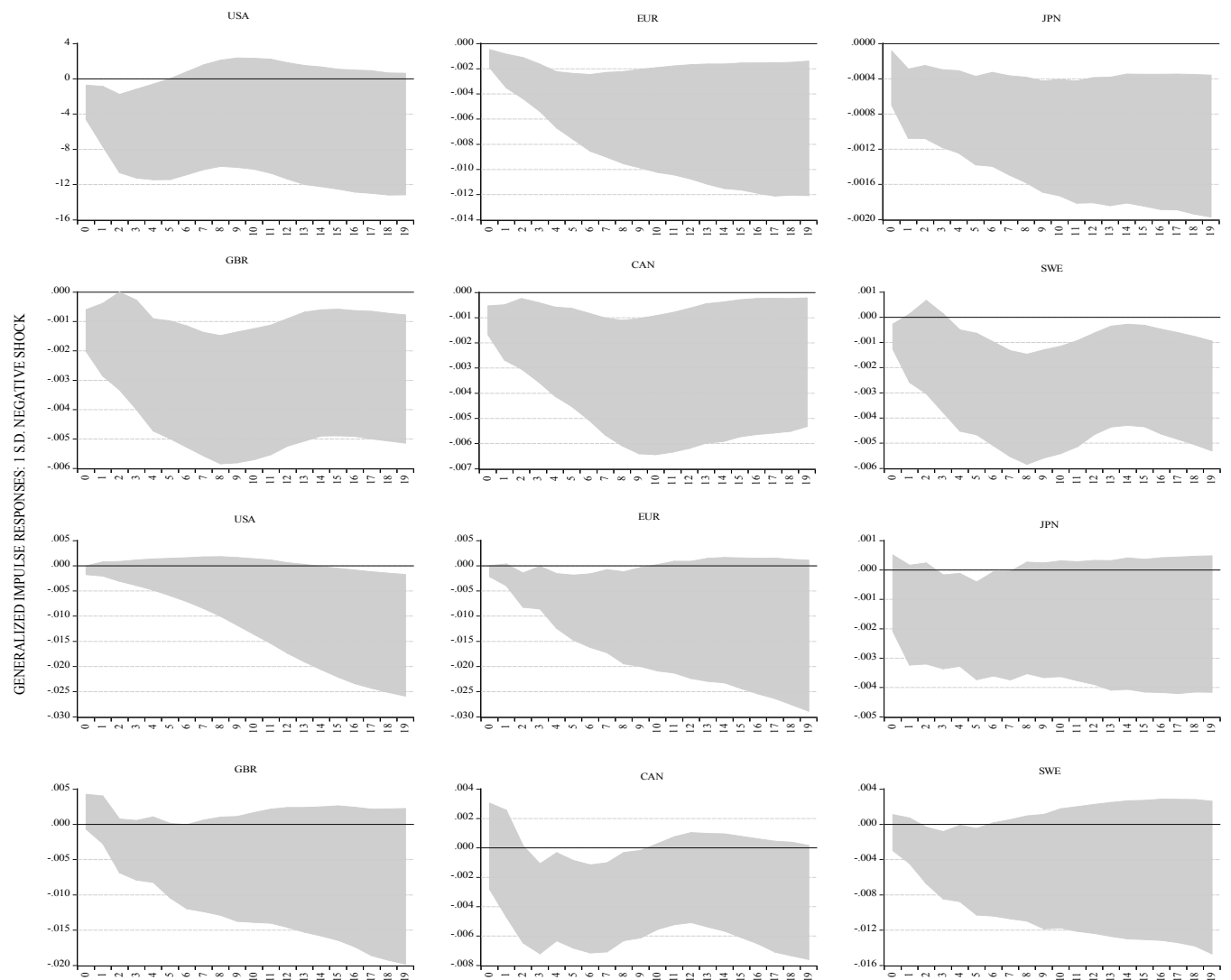
Figure 7B Impulse Responses to a Negative Loan Demand Shock from the UNITED STATES
