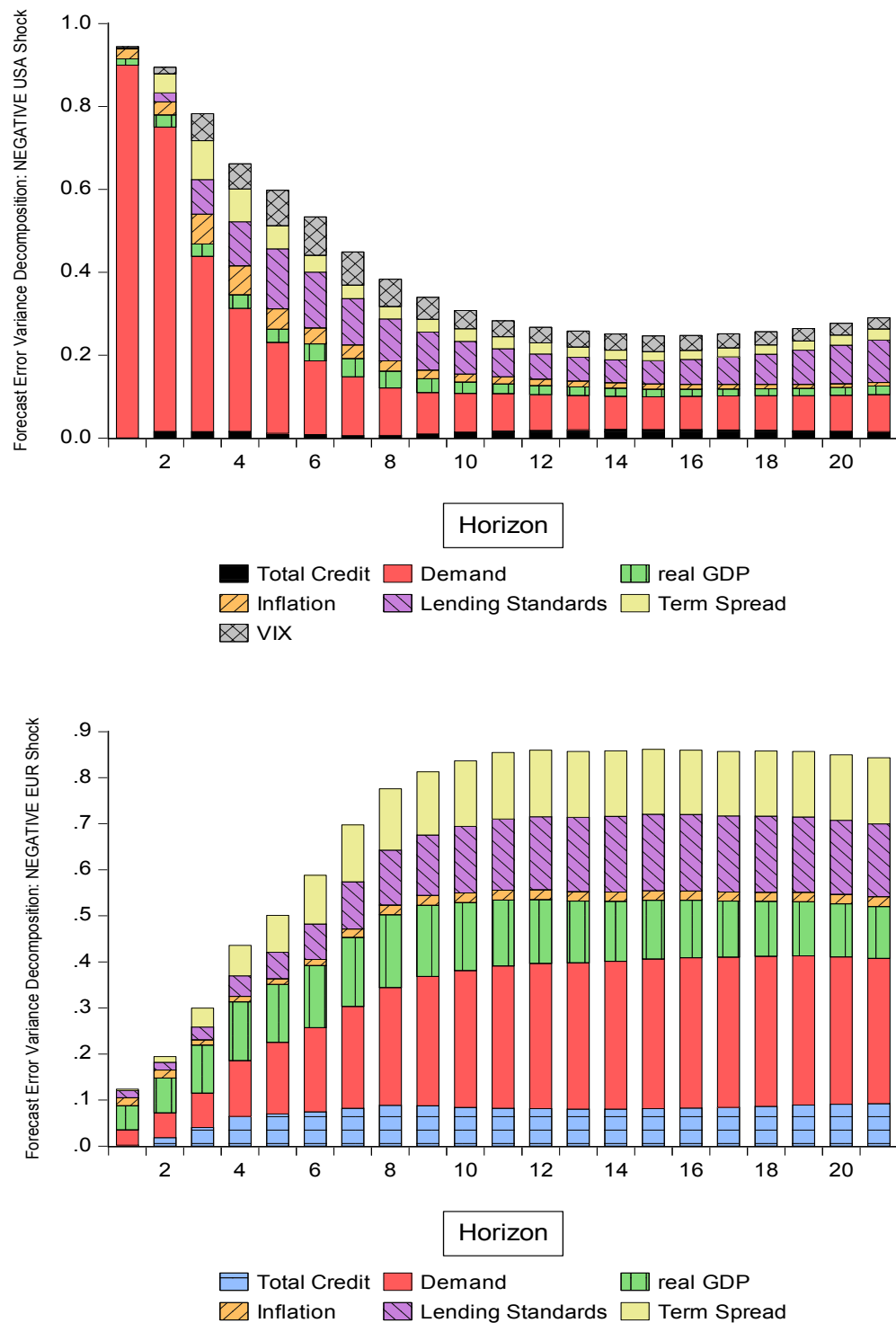
Figure 10 Forecast Error Variance Decompositions: Negative Loan Demand Shock
