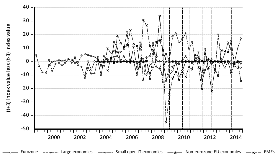
Figure 1B - Expected Movements in Lending Standards – Global
