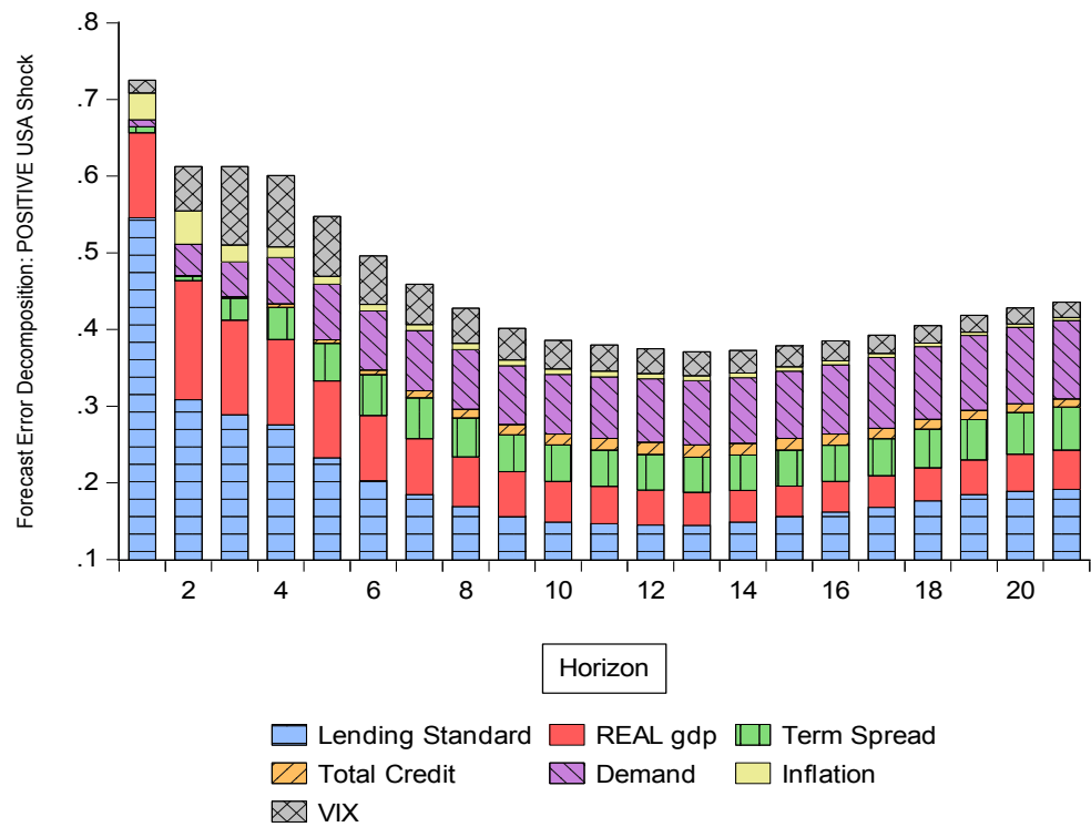
Figure 9 Forecast Error Variance Decompositions: Positive Lending Standards Shock
