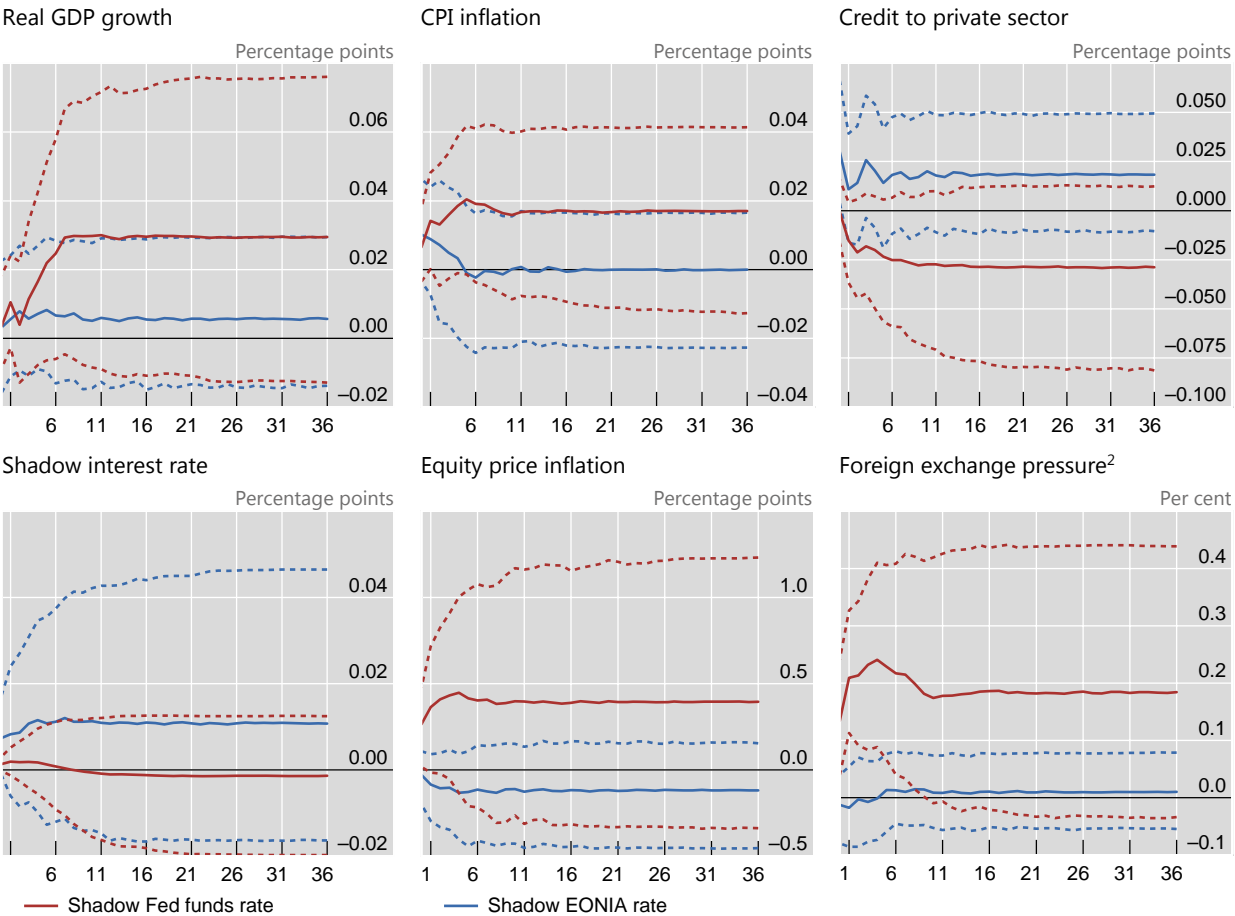
Trans-Atlantic impacts
