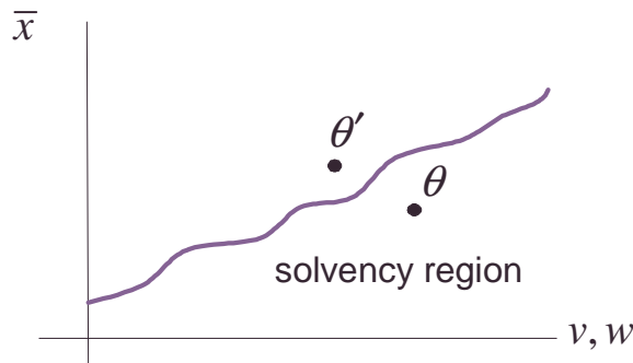
Figure 2: Solvency region for \theta
