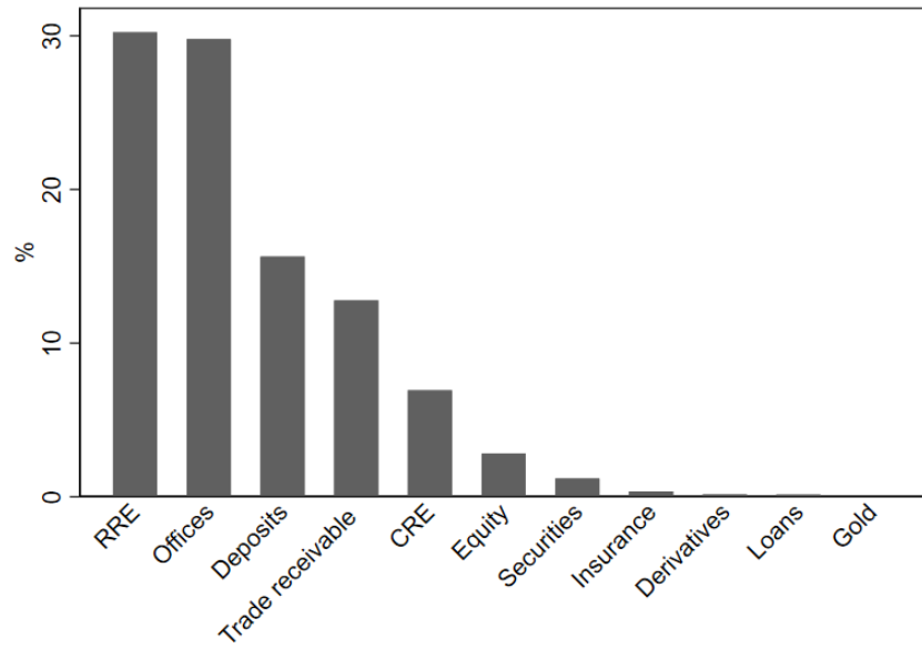
Figure 5: Collateral distribution
