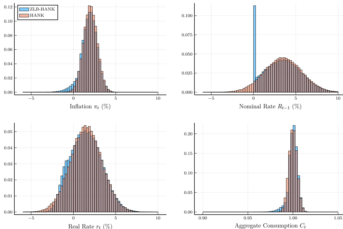
Figure 3: Ergodic Distributions.
