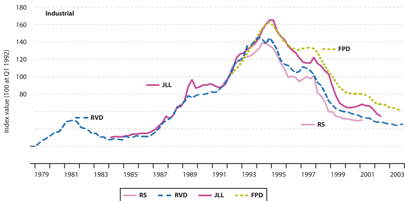
Figure 10.17 Industrial indices
