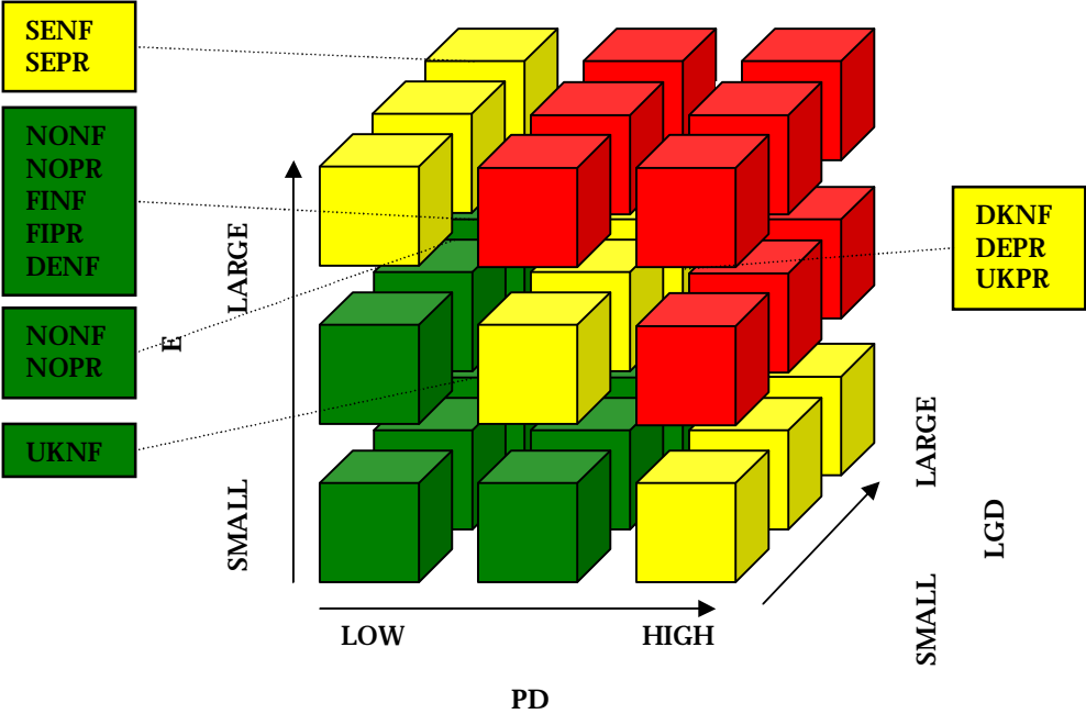
Figure 4. Credit risk cube; three-dimensional, three levels (3x3x3)
