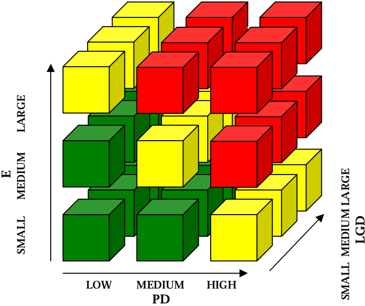
Figure 3. Credit risk cube; three-dimensional, three levels (3x3x3)
