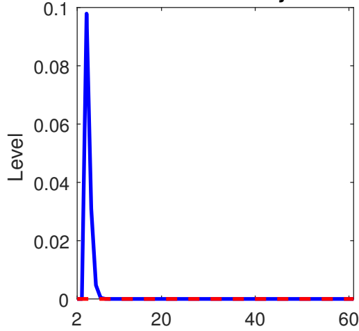
Run Probability
