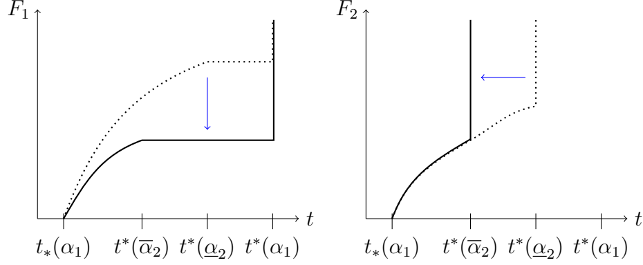
Figure 3: The mixing distributions of regulator 1 and regulator 2 as regulator 2 becomes more growth focused
