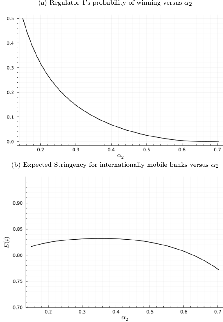
Figure 4: The impact of growth-focused country becoming even more growth focused
