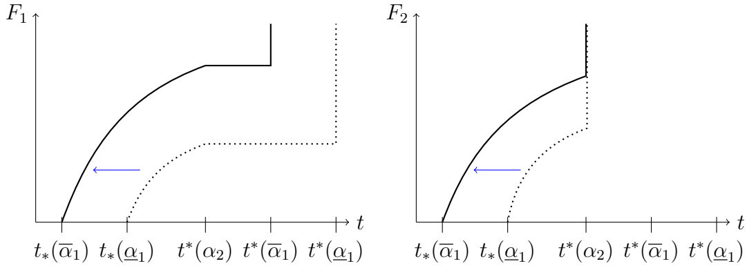
Figure 5: The mixing distributions as regulator 1 pivots to become more growth focused Notes: The dotted line represents the distribution under \underline{\alpha}_1 while the solid line represents the distribution under \bar{\alpha}_1 when regulator 1 is more growth focused. That lower levels of regulatory stringency are delivered is evident.
