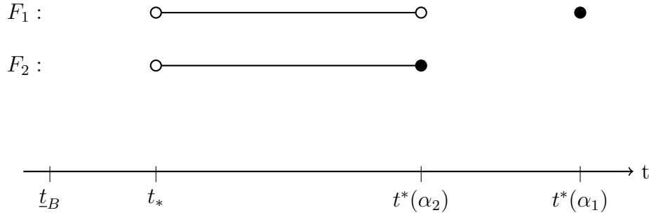
Figure 1: The support of the mixing distribution established in Theorem 2
