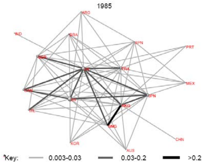
Chart 1: Global Financial Network: 1985
