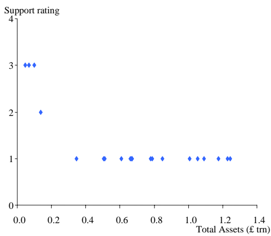
Chart 10: Global Banks' Size and Government support (a)
