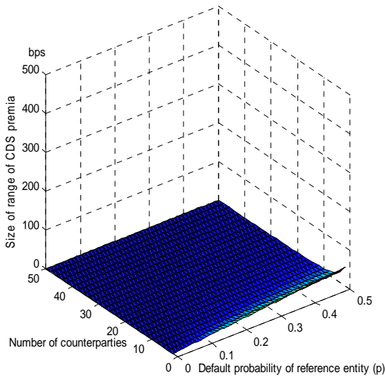
Chart 4: CDS Premia and Network Uncertainty – Pre-crisis
