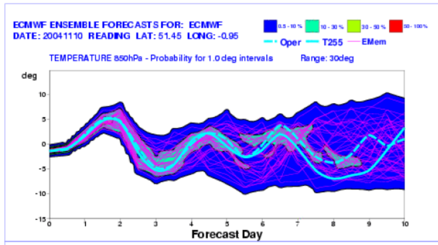
Chart 7: Temperature forecast on 10 November 2004
