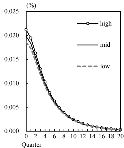
(7) Earnings per labor input in sector X
