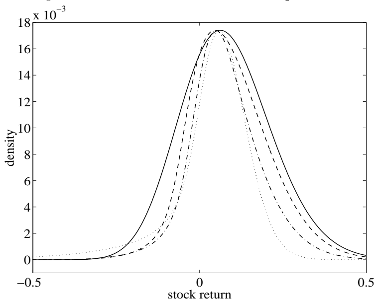
Figure 9: Stock return distribution in equilibrium
