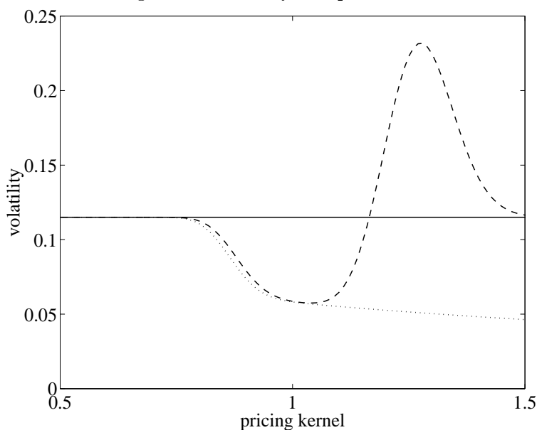
Figure 4: Volatility in equilibrium
