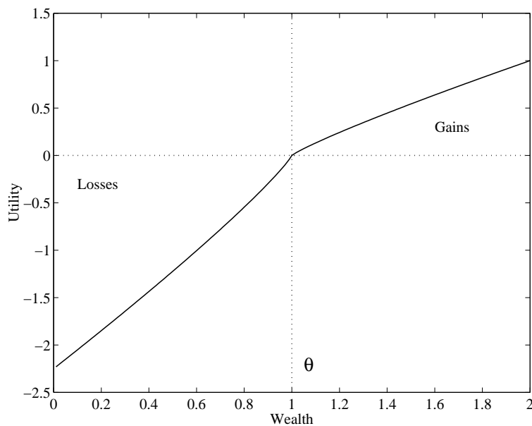
Figure 11: Utility function of prospect theory
