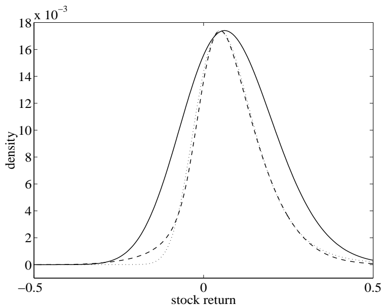
Figure 13: Stock return distribution in equilibrium
