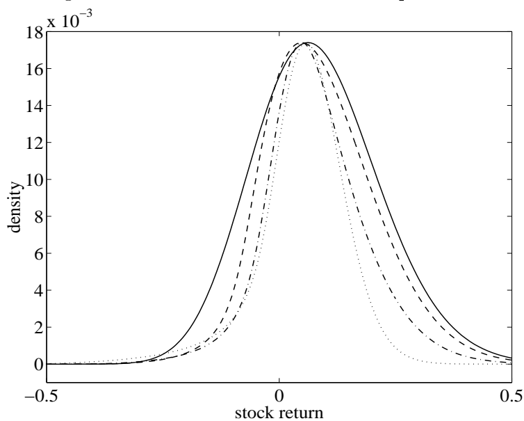
Figure 8: Stock return distribution in equilibrium
