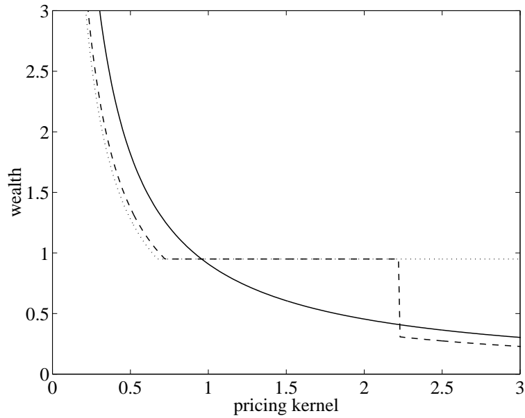
Figure 1: Wealth at time T=1
