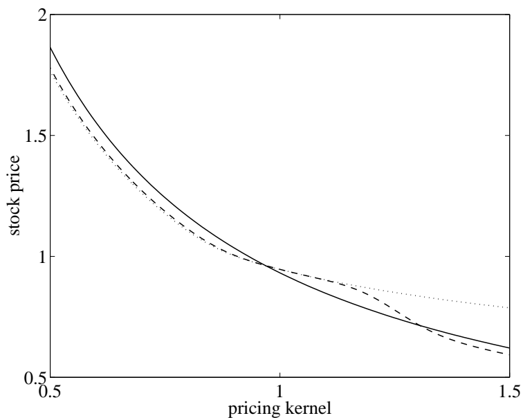
Figure 6: Stock price in equilibrium
