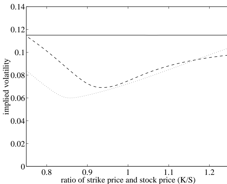
Figure 14: Implied volatility of equilibrium option prices
