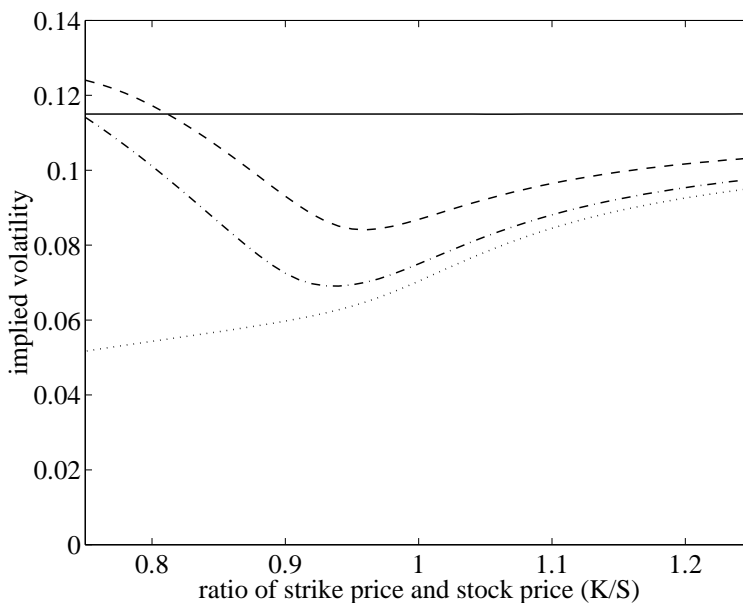
Figure 10: Implied volatility of equilibrium option prices
