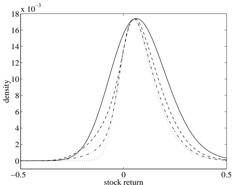
Figure 7: Stock return distribution in equilibrium
