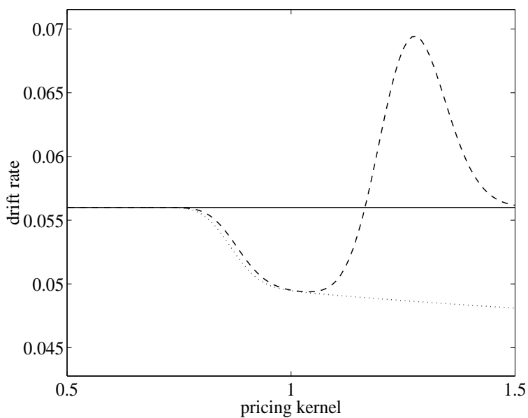
Figure 5: Drift rate in equilibrium
